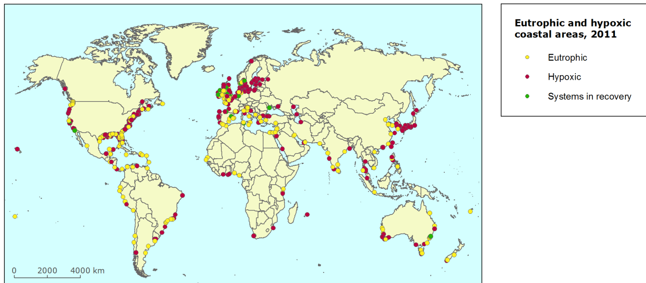
Figure 10.11 Eutrophic and hypoxic coastal areas, 2011
