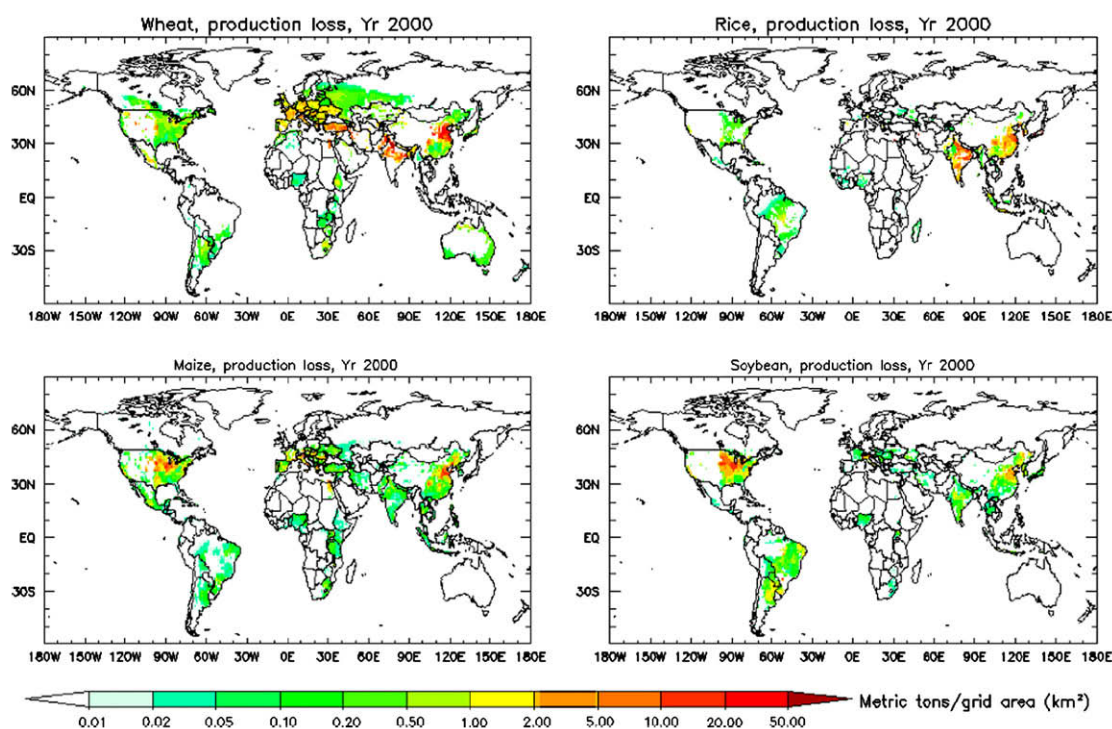
Figure 10.12 Modelled crop production loss due to O 3 for wheat, rice, maize and soybeans, 2000
